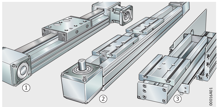
Figure 4 Linear actuators with additional function
